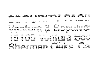
Figure 8. Binary image
